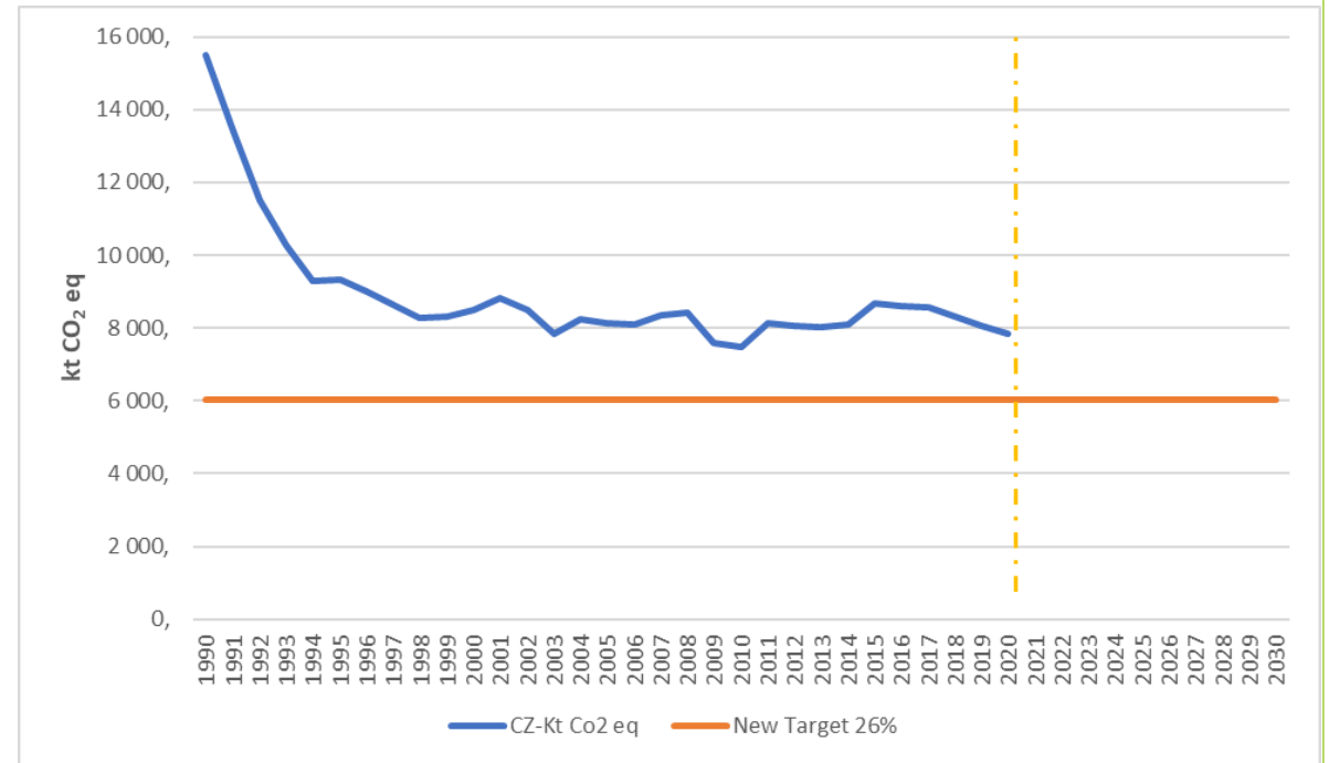
Agriculture GHG emissions for the CZ in kt CO 2 eq 1990-2020
