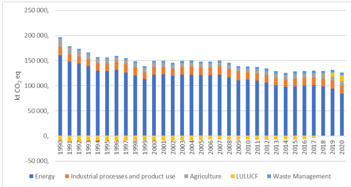
CZ GHGs Emission by source sector in kt CO 2 eq.
