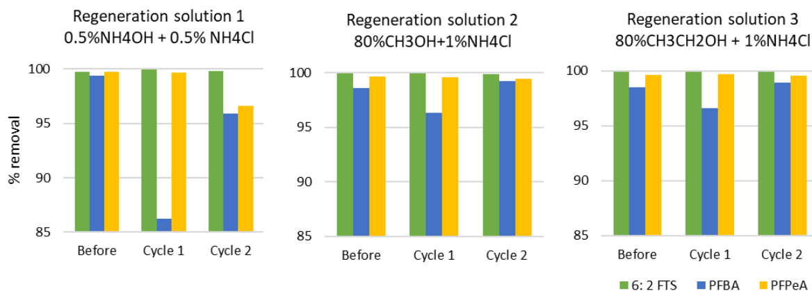
Fig. 2 Adsorption capacity of the resin PFA694E after two regeneration cycles with three different regeneration solutions.
